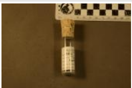
MWC 9510 (9510)
